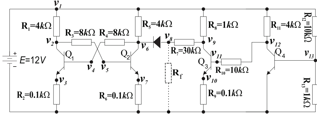
Figure 2: Circuit under test (contains three operating points). R_f = 11k\Omega models a possible fault between node v_8 and ground.
