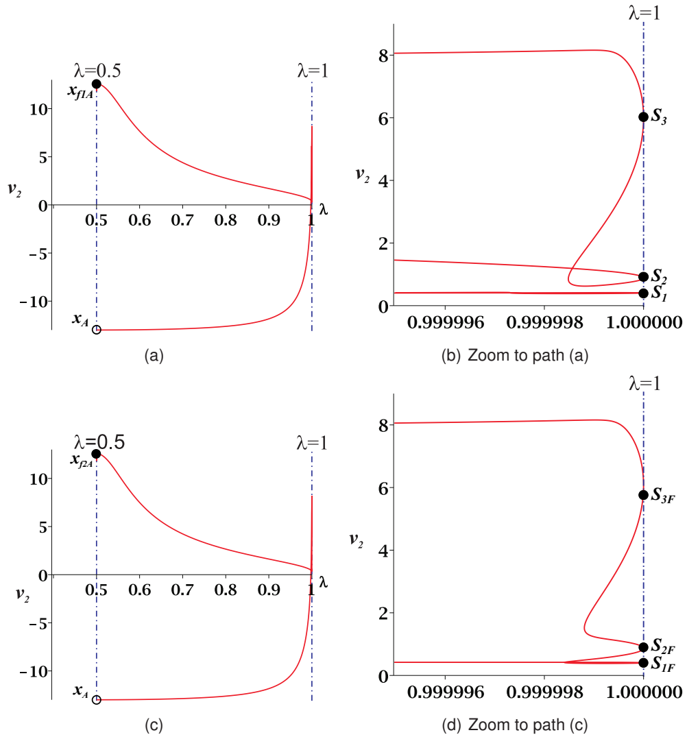
Figure 3: Homotopy paths \lambda - v_2 for initial point at x_A : (a),(b) the fault-free circuit, and (c),(d) fault circuit.
