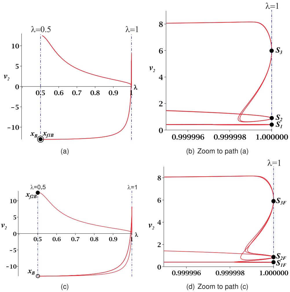
Figure 4: Homotopy paths \lambda - v_2 for initial point at x_B : (a),(b) the fault-free circuit, and (c),(d) fault circuit.
